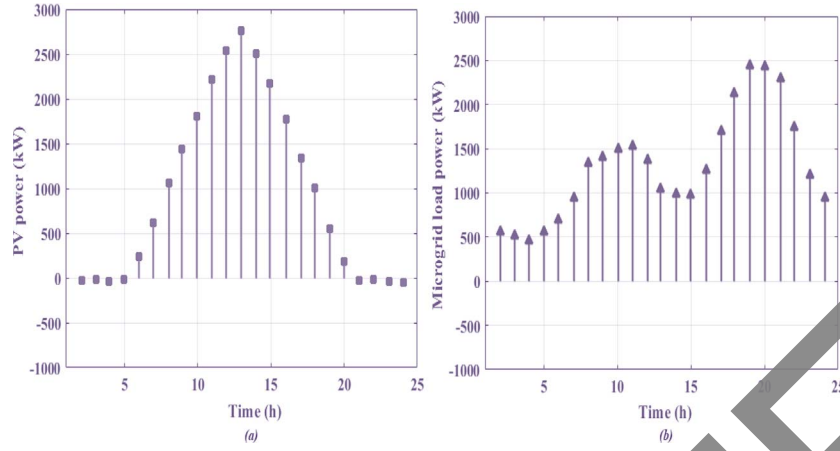
Fig. 10. Case 3. (a) PV power and (b) demand of microgrid.
