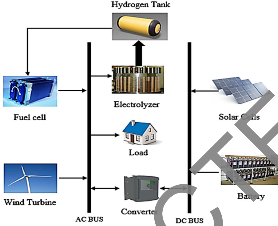
Fig. 1. Microgrid configuration.
